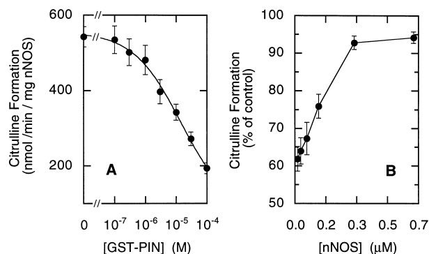
Fig. 1. Inhibition of rat nNOS by GST-PIN. NOS was preincubated with GST-PIN for 30 min at 37°C, in 55 mM triethanolamine-HCl, pH 7.0/0.55 mM CaCl 2 /0.22 mM CHAPS with L-Arg (110 μM; including L-[2,3,4,5- 3 H]Arg), H 4 biopterin (11 μM), NADPH (220 μM), FMN (5.5 μM), and FAD (5.5 μM). NOS reactions were started by adding 10 μl CaM (0.1 mg/ml). Error bars denote S.E.M. of three experiments. A: Dependence of inhibition on PIN concentration at fixed nNOS concentration of 63 nM. The data were fitted to a Hill-type equation. B: Dependence of inhibition on nNOS concentration at fixed PIN concentration (3 μM).
